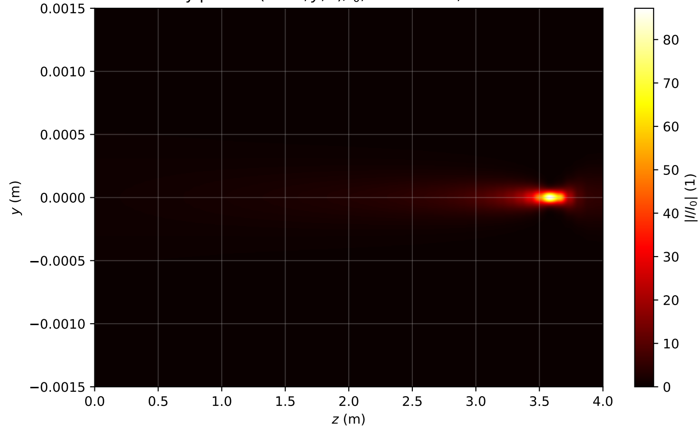
Intensity profile I(x=0, y, z)/I_0 , P_{in}=1.1P_{cr} , artificial time
